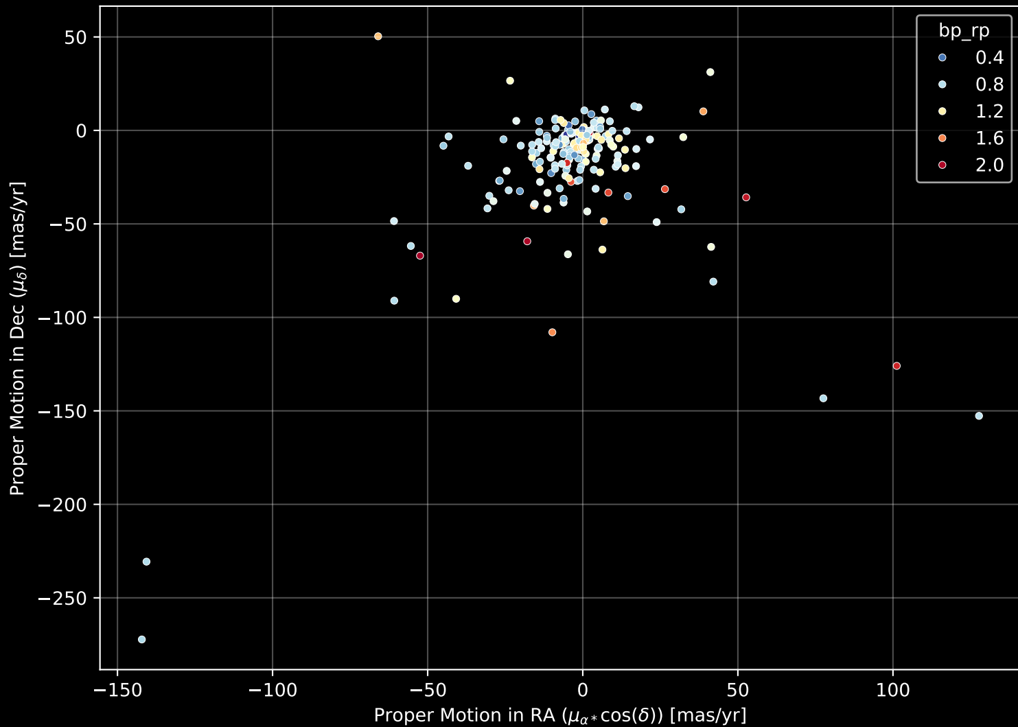
APOGEE DR17 Field: [170+31_MGA] Proper Motion Diagram (n= 198)
