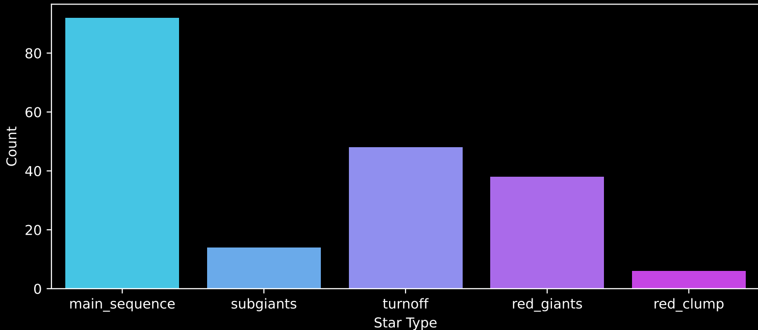
APOGEE DR17 Field: [170+31_MGA] Count plot of Star Type
