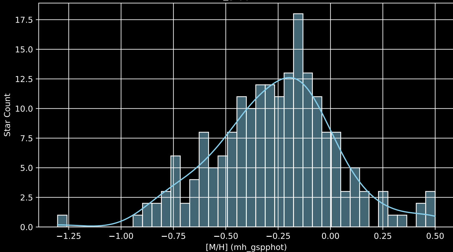
APOGEE DR17 Field: [170+31_MGA [M/H] (mh_gspphot) (n= 196)
