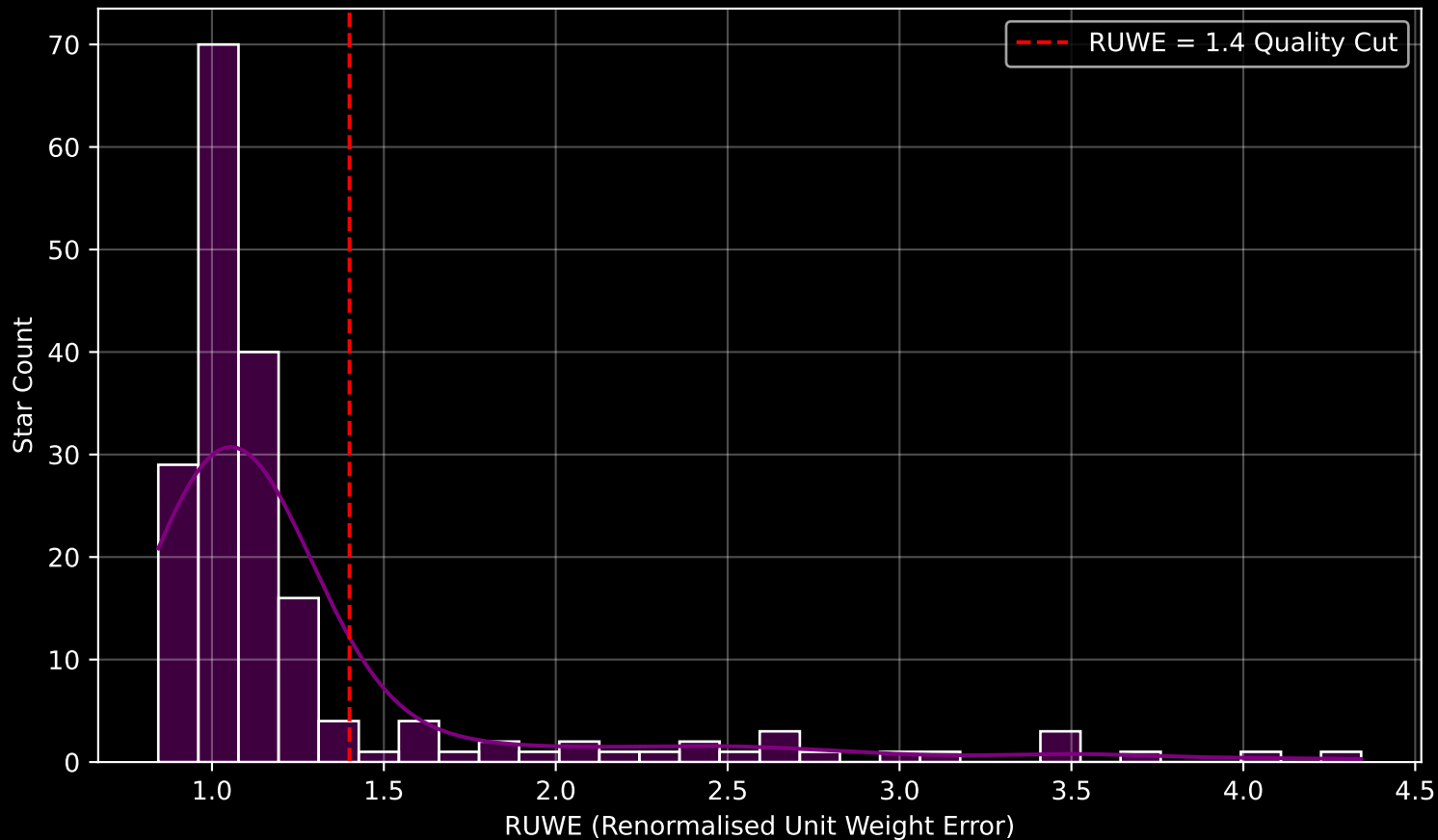
GAPOGEE DR17 Field [170+31_MGA] RUWE Distribution (n= 187)
