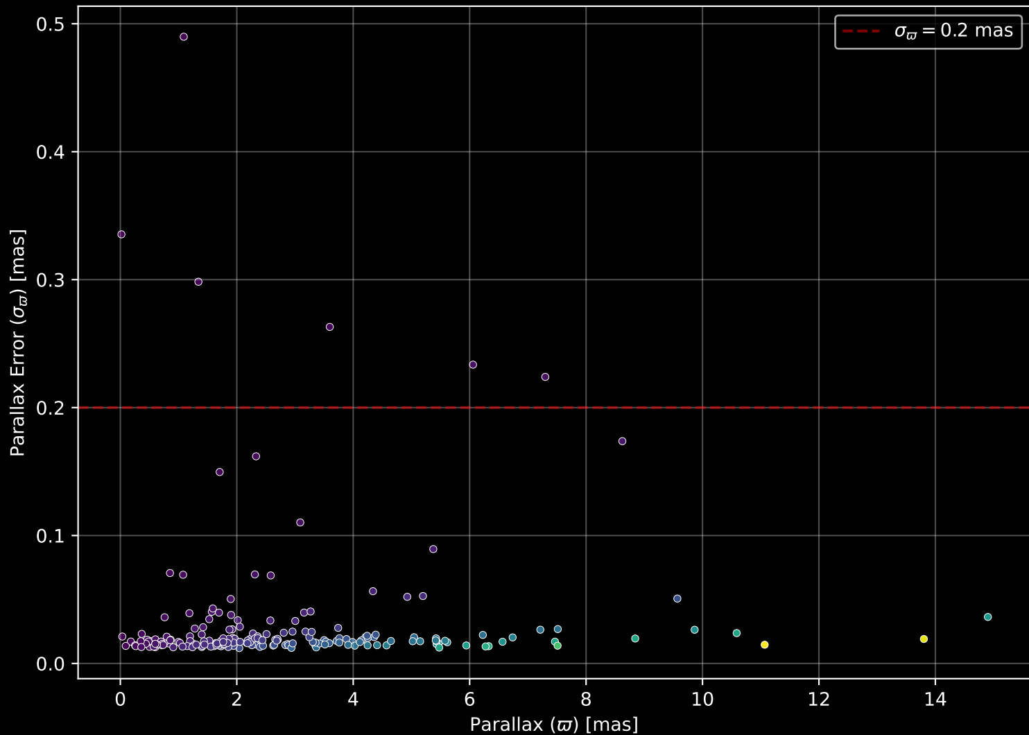
APOGEE DR17 Field: [170+31_MGA] Parallax Quality (n= 198)
