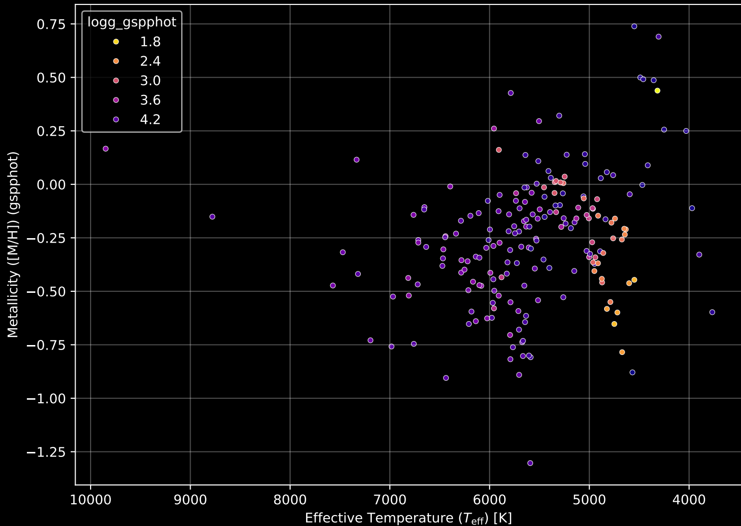
APOGEE DR17 Field: [170+31_MGA] Stellar Population Parameters (n= 198)
